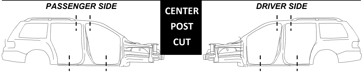
STANDARD POST CUT = 6 INCHES BOTH DIRECTIONS AT TOP POST, HALFWAY THROUGH EACH BOTTOM DOOR OPENING
