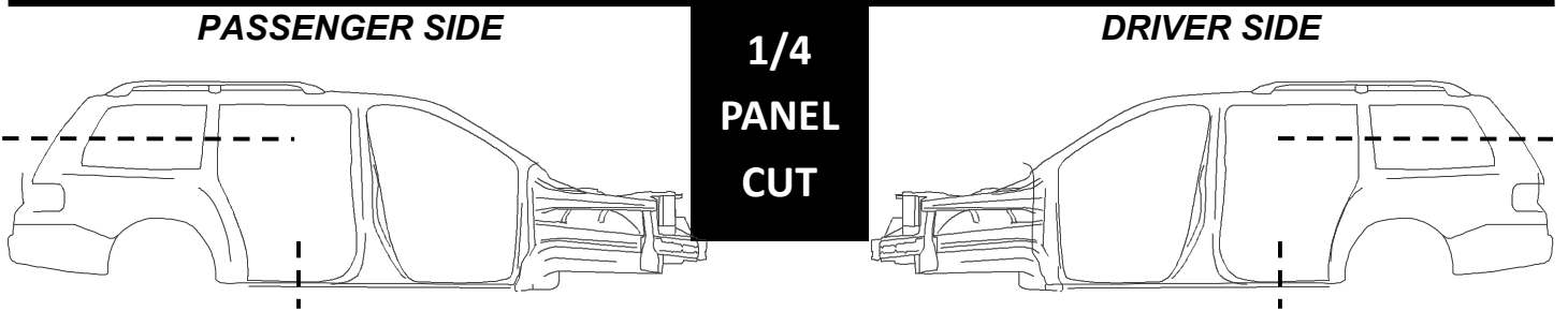
STANDARD 1/4 PANEL CUT = HALFWAY DOWN THE SAIL PANEL AND HALFWAY THROUGH EACH BOTTOM DOOR OPENING.
